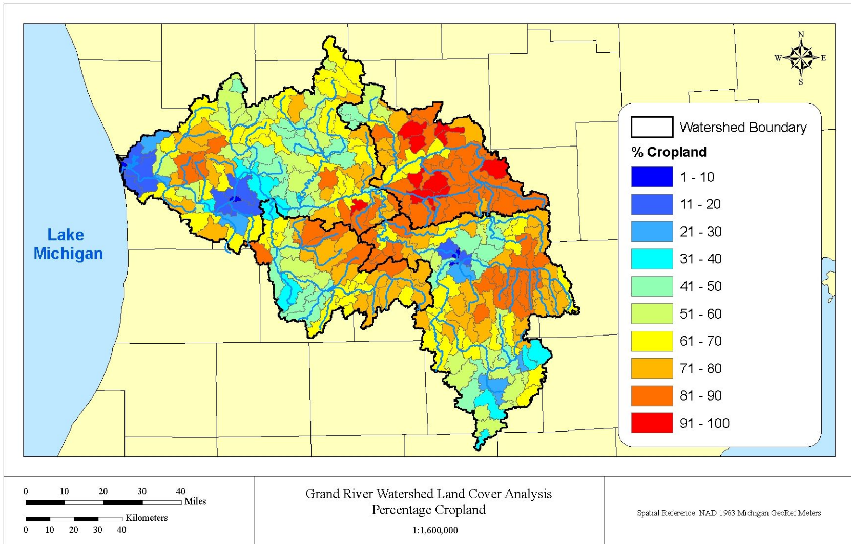
Figure 3.4 Cropland Percentage for Each HUC14 Watershed
