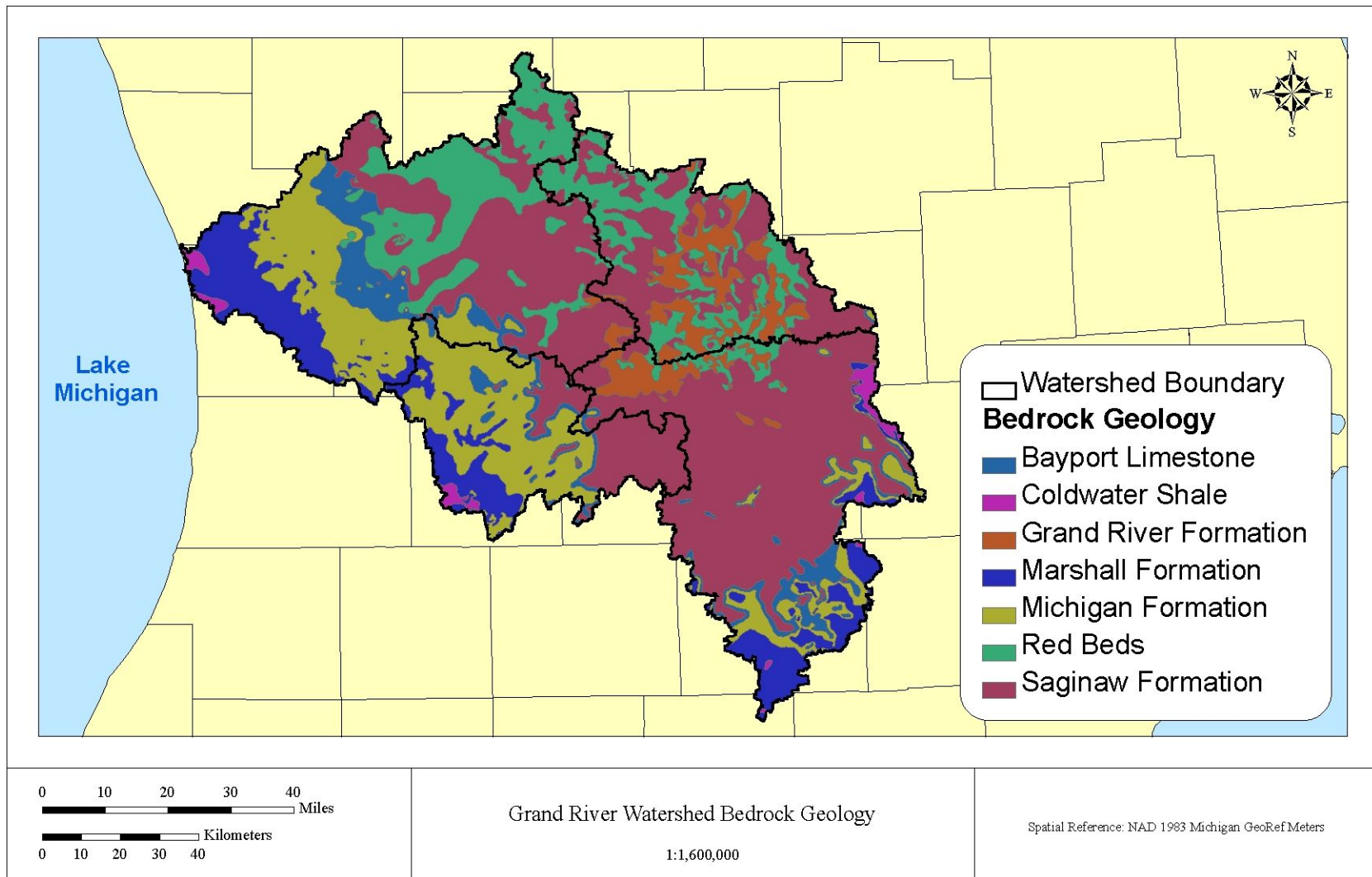
Figure 3.19 Grand River Watershed Bedrock Geology
