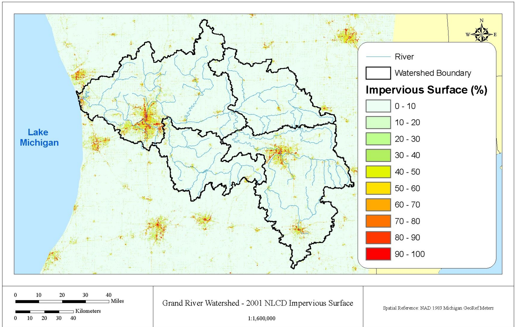
Figure 3.8 Impervious Surfaces in the Grand River Watershed
